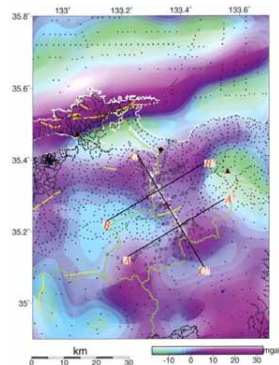
Fig. 3. Band-pass filtered (wavelength of 20-30 km) Bouguer anomaly map overlaid with epicenters of aftershocks (white dots) and locations of visited (black dots) and new (open circles) gravity stations. Density for reduction is assumed to be 2.67 g/cm 3 . White, green and yellow solid lines indicate the coastline, prefectural boundary and active faults, respectively. Black lines are the lines where subsurface structures are analyzed.
