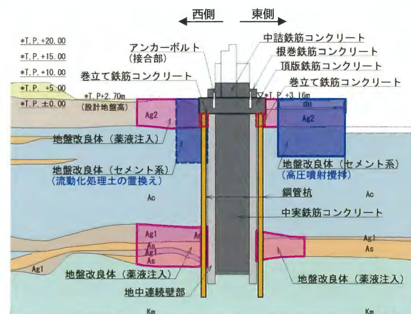
(c)-(c)断面図
