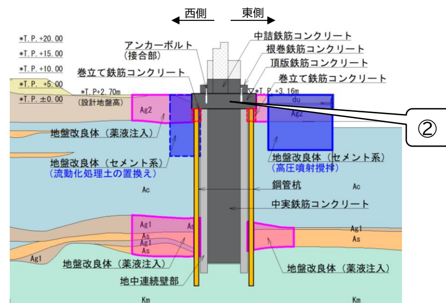
(c)-(c)断面図
