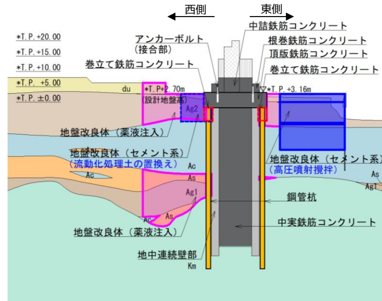
(c)-(c)断面図
