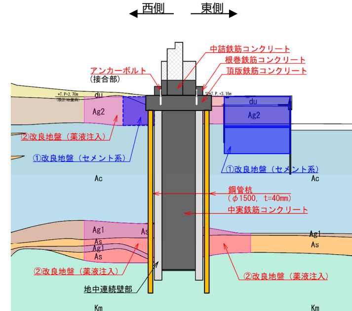
(c)-(c)断面図※1
