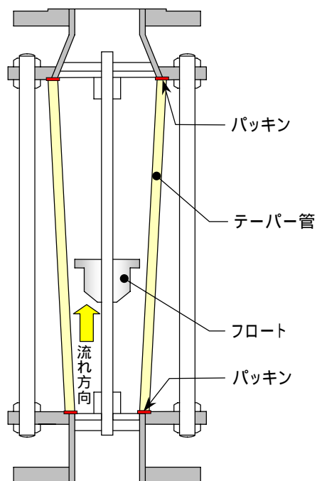
[流量計断面図]
